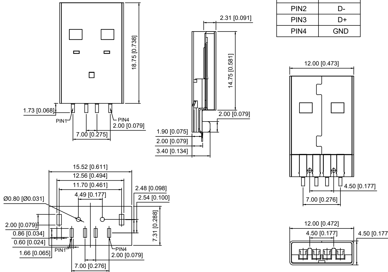
PCB LAYOUT
