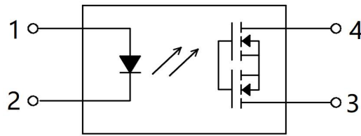
Pin Configuration 1.Anode 2.Cathode 3.Drain1 4.Drain2
