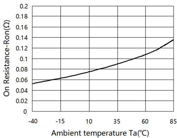
Fig.3 On Resistance vs Ambient temperature
