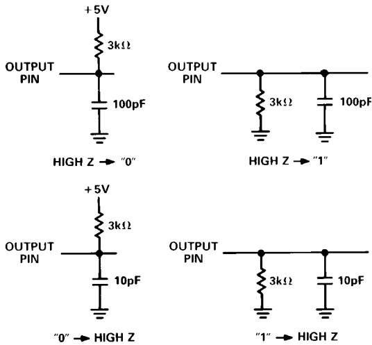
Figure 22. Output Loads
