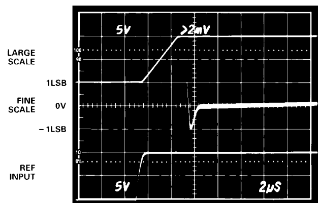
Figure 5. Settling Time; Input Bits Fixed, Reference Switched
