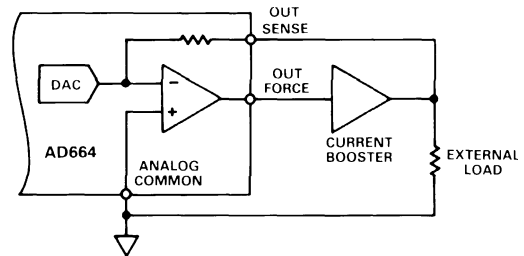
Figure 3. Current-Boosting Scheme
