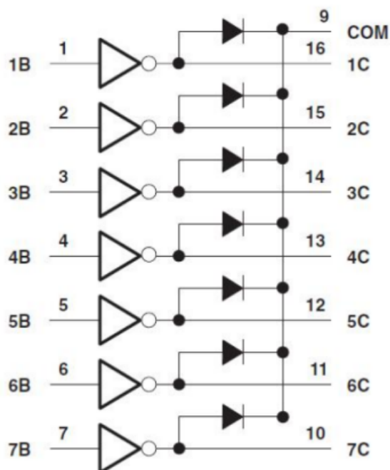
LOGIC DIAGRAM
