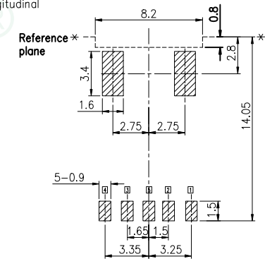
Recommended PCB Layout Tolerance: ±0.1(Top view)
