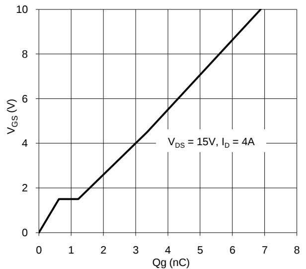
Figure 22. Gate Charge
