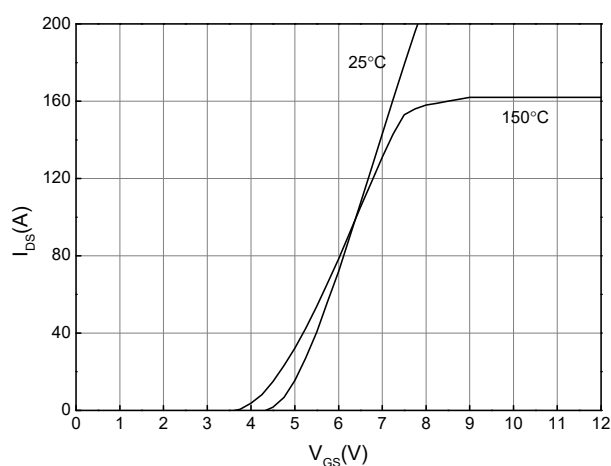
Figure 3. Typical Transfer Characteristics ( V_{DS} = 20\text{V} , Parameter: T_J )
