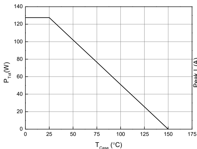
Figure 9. Power Dissipation
