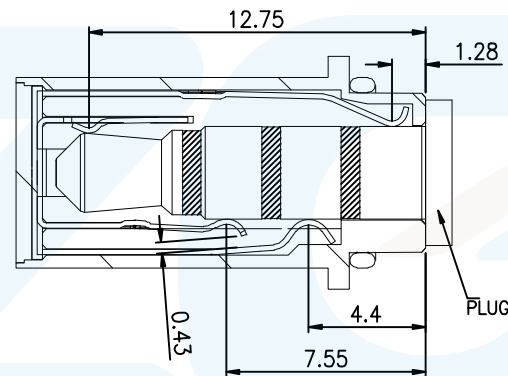
SEC:A-A Image of plug match with contact point
