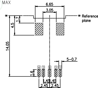
Recommended PCB Layout Tolerance: ±0.1(Top view)
