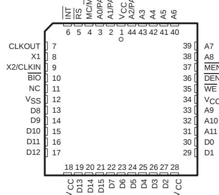
TMS320C16 PG Package (Top View)
