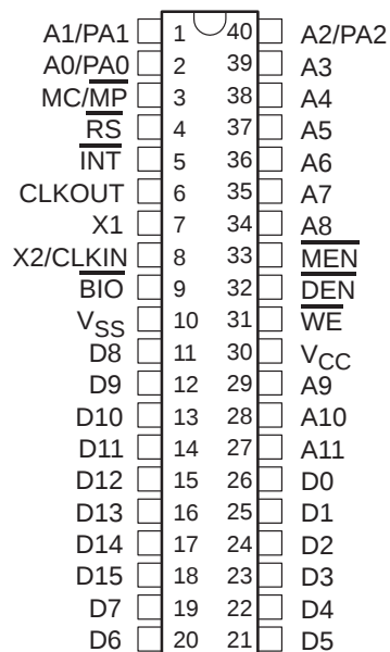
TMS320C15/E15/LC15/P15 N/JD Package (Top View)
