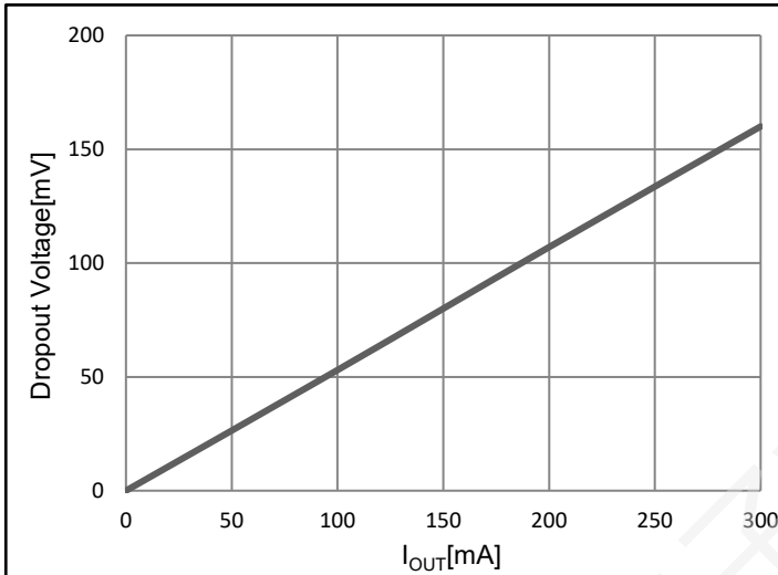
5. Dropout Voltage ( V_{OUT} = 95\% \times 2.8V , I_{OUT} = 0 \rightarrow 300mA )
