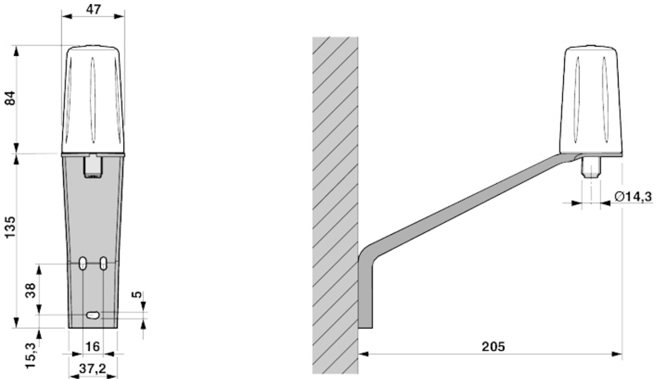
Dimensional drawing
