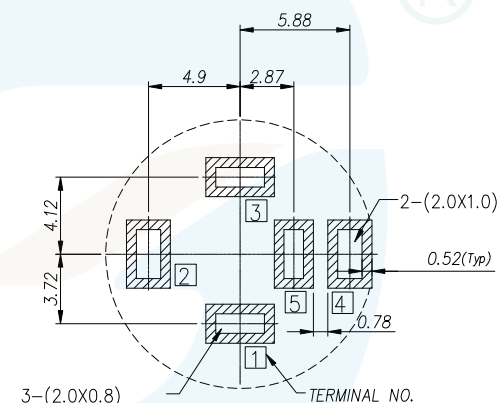
RECOMMENDED PCB LAYOUT(t=1.6) UNSPECIFIED TOLERANCE: ±0.05 (BOTTOM VIEW)
