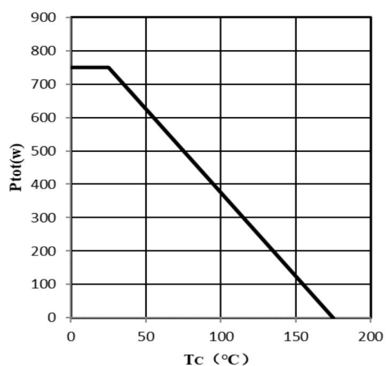
Fig 2. Power dissipation as a function of case temperature ( T_j \leq 150^{\circ}\text{C} )
