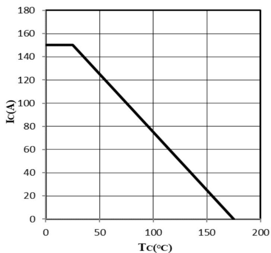
Fig 1. DC Collector current as a function of case temperature ( V_{GE} \geq 15\text{V} , T_j \leq 150^{\circ}\text{C} )
