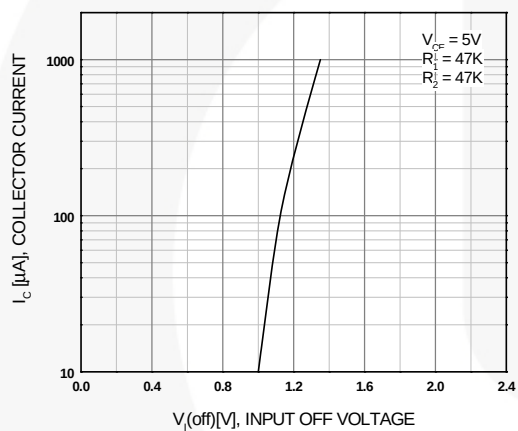
Figure 3. Input-Off Voltage
