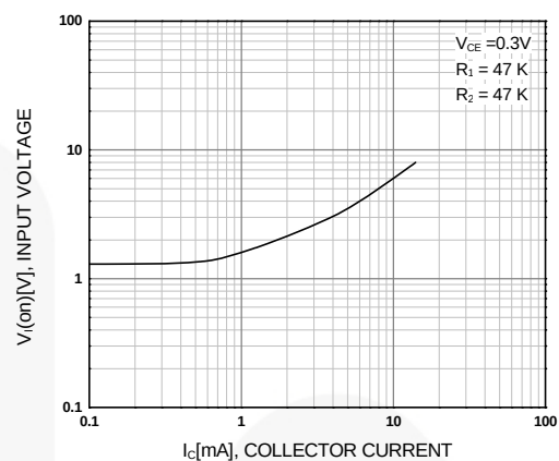
Figure 2. Input-On Voltage
