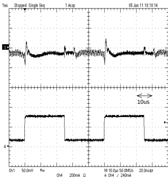
Figure 20. Load transient response 50mA to 350mA t_r=t_f=100\text{ns} , MODE : Low
