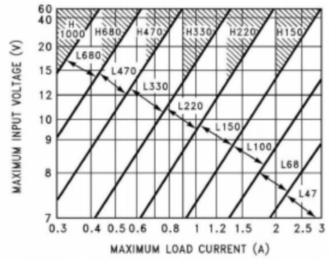
LM2576HV-5.0
