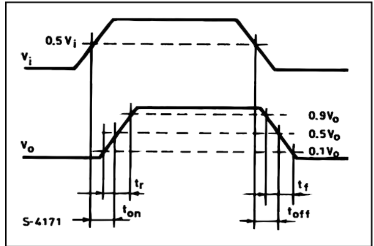
Figure 1: Switching Times
