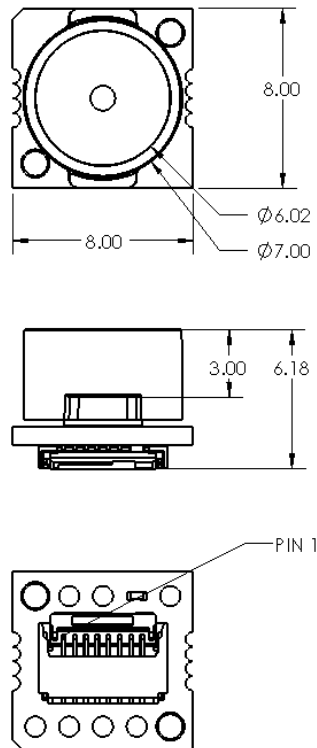
Figure 4. Dimensions of the EV_MOD_CH201 assembly
