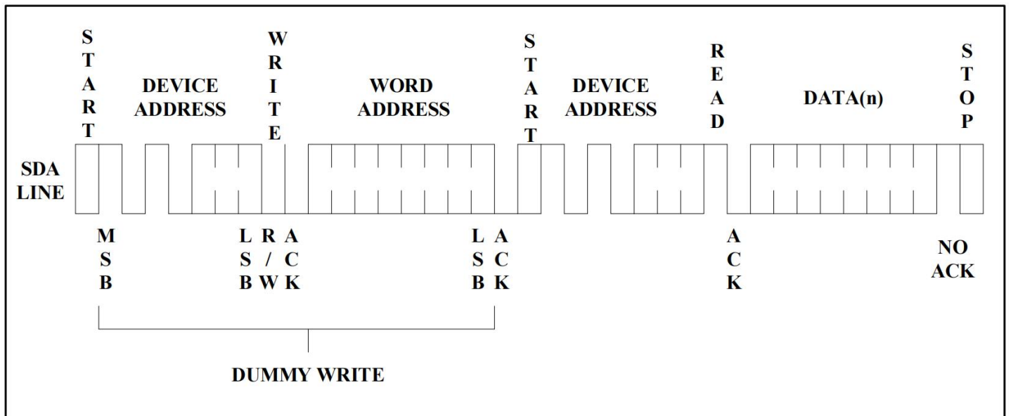
Figure 10. Sequential Read
