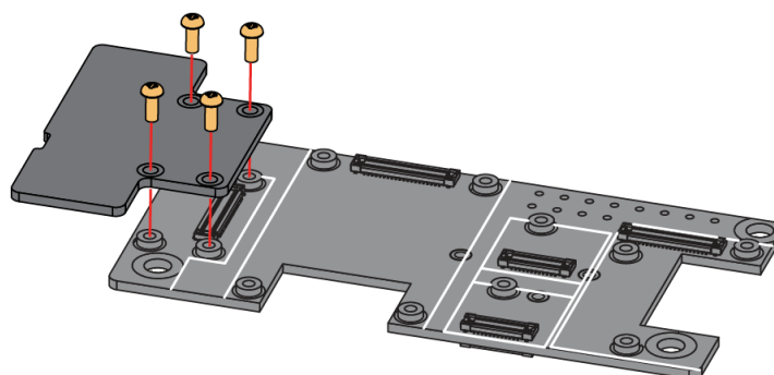
Figure 2: RAK19012 mounting mechanism on a WisBlock Base module
