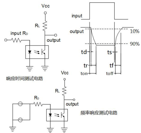
Fig.10 Switching Time Test Circuit & Waveforms
