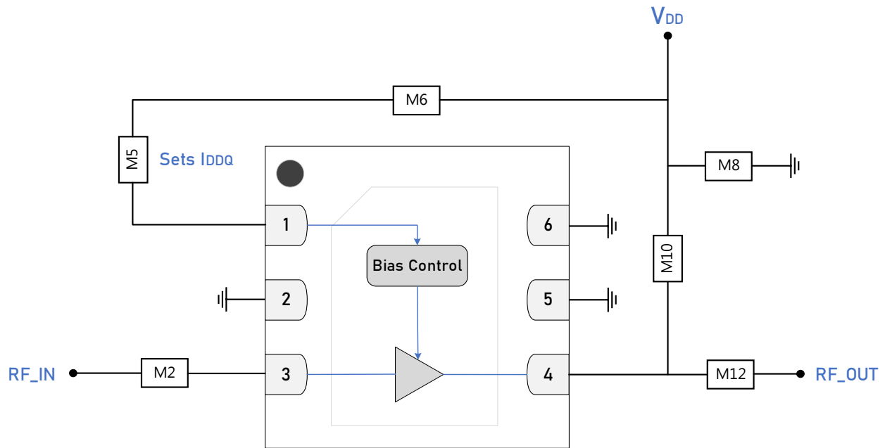
GRF2013W Standard Evaluation Board Schematic
