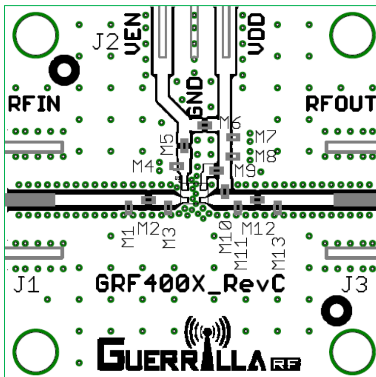
GRF2013W Evaluation Board Assembly Diagram
